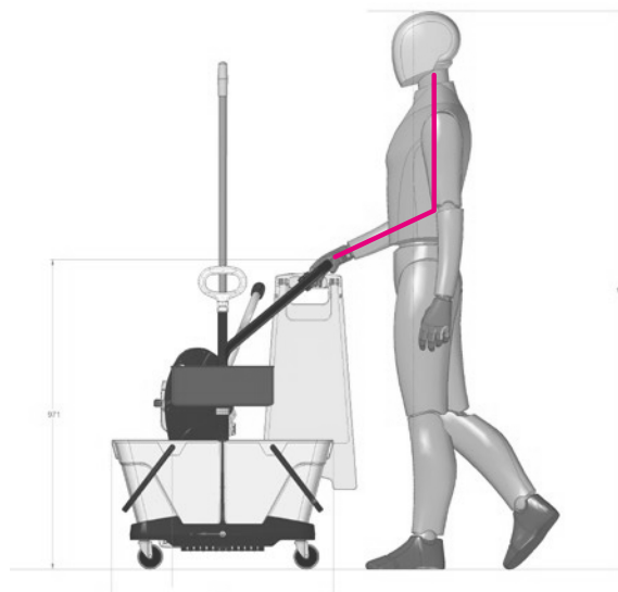
50th percentile male | inclination of the forearm during pushing.
