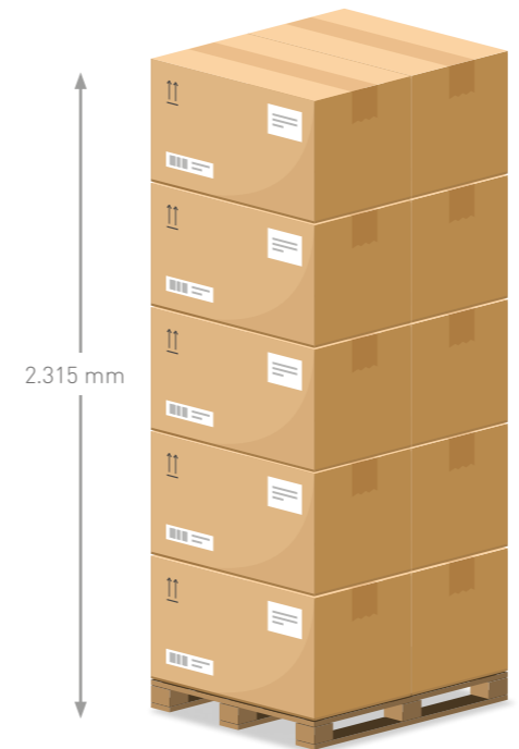
2P's Palettierung 783mm x 433mm x 516mm = 0,184mc
